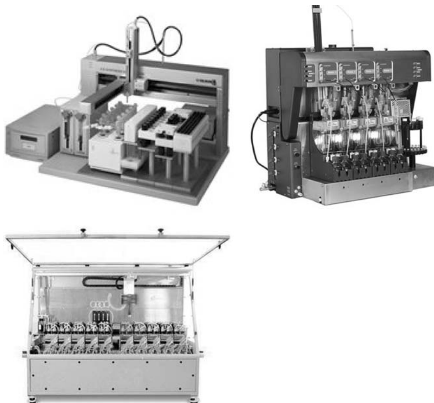
Fig. 8 Synthesizers for process development: ReactArray SK215, Argonaut-Biotage Advantage 3400, and Chemspeed Accelerator PXT100.
